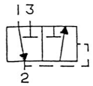
QUICK EXHAUST
